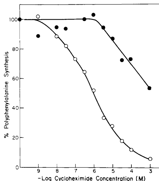
FIGURE 2: Cycloheximide concentration curves. Polyphenylalanine synthesis was measured at the indicated cycloheximide concentrations in the absence of P factor (●) or in the presence of 0.9 μg of P factor (○). Other factors are as indicated in Figure 1B. Uninhibited values were 1.45 pmol in the presence of P and 1.57 pmol in the absence of P.
