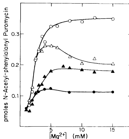
FIGURE 4: Effect of MgCl_2 concentration on the factor dependence of N -AcPhePuro synthesis. The reaction was carried out for 3 min at 30 °C in the presence of (○) 0.08 µg of EF-2, 0.2 µg of EF-3, and 0.3 µg of P factor; (△) EF-2 and P factor; (▲) EF-3 and P factors; (●) P factor. Activity in the absence of P factor was less than 0.1 pmol at all MgCl_2 concentrations.
